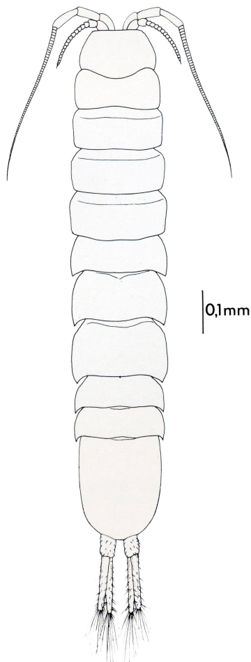
Fig. 3. Stenasellus migiurtinicus (Isopoda: Stenasellidae) described in 1974 from underground waters of NW Somalia (from Messana, Chelazzi & Lanza, 1974; almost all the appendices are not represented).
